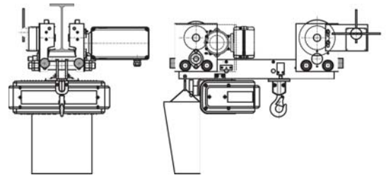
Low Headroom Trolley
